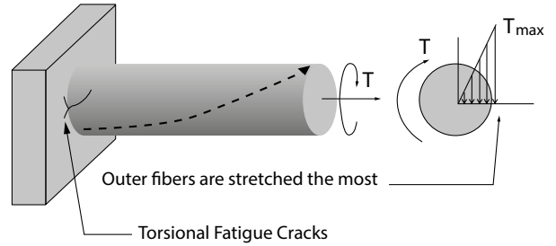
Fig. 5-1 Torsional Loading
