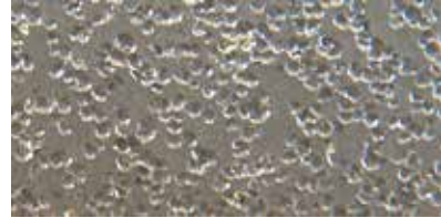
Fig. 11-8B Incomplete Shot Peening Coverage
