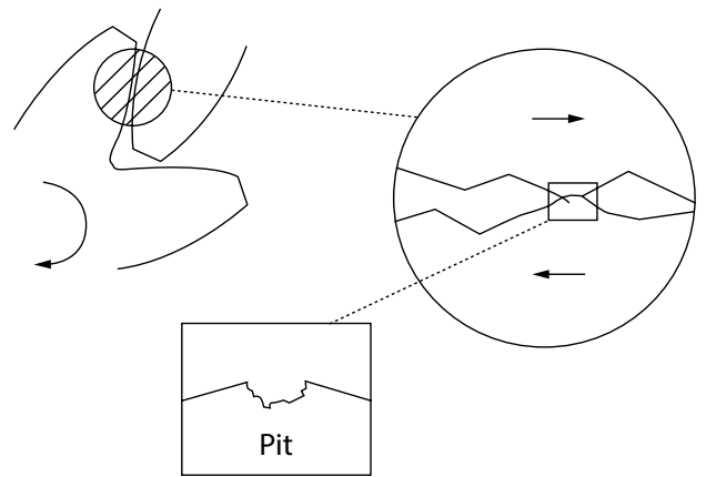
Fig. 7-3 Pitting Failure Schematic
