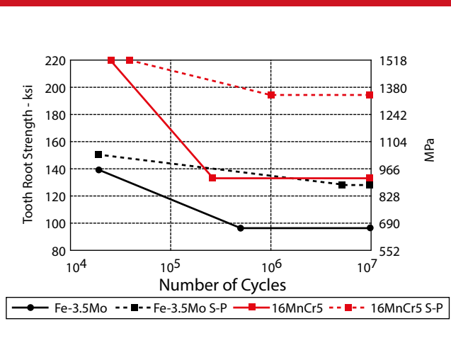
Fig. 2-6 Fatigue Life Curves Comparing a Reference (16MnCr5) Wrought Steel to a 7.5 g/cm 3 Powdered Metal (Fe-3.5Mo) with and without Shot Peening.
