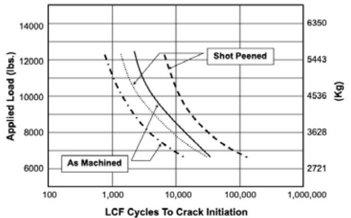
Fig. 2-5 LCF Benefits from Shot Peening Notched Ti8-1-1
