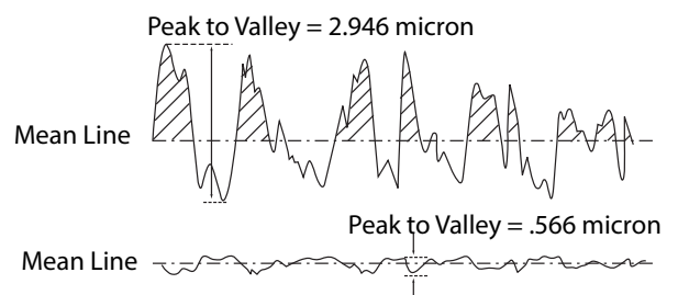
Fig. 10-15 Surface Roughness After Shot Peening and After C.A.S.E. SM Finishing
