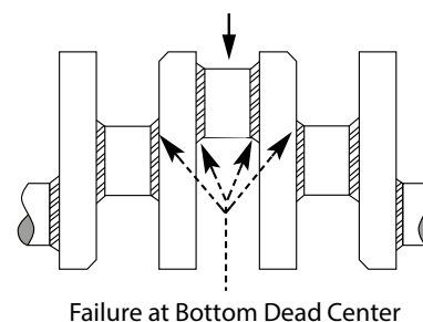
Fig. 4-6 Crankshaft Schematic
