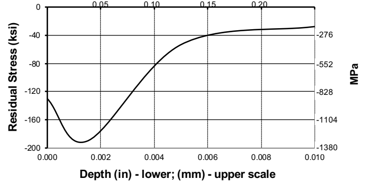
Fig. 4-4 Typical Carburized Gear Residual Stress Profile
