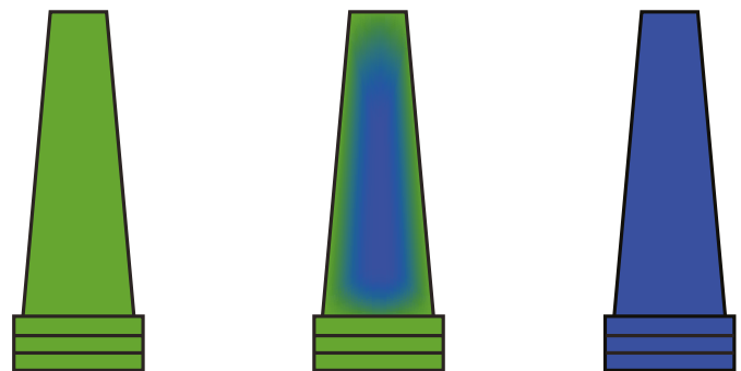
Fig. 11-9A Peenscan® Coating prior to Shot Peening Fig. 11-9B Partial removal of Peenscan® indicating incomplete coverage Fig. 11-9C Complete removal of Peenscan® indicating complete coverage
