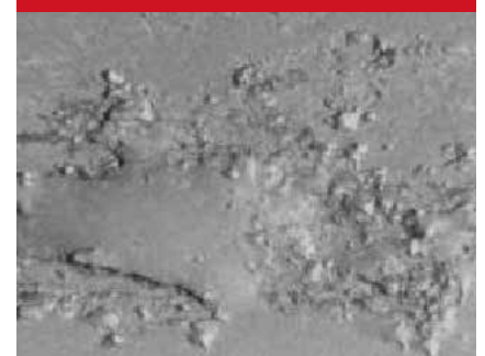
Fig. 10-8 Exfoliation Corrosion
