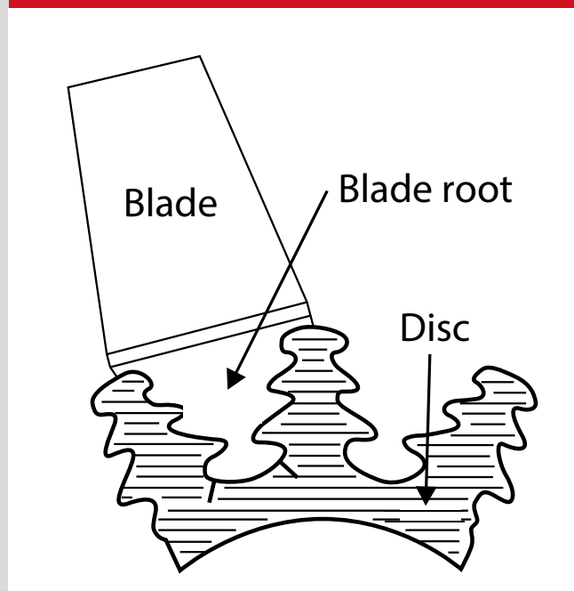
Fig. 7-2 Turbine Blade and Disc Assembly
