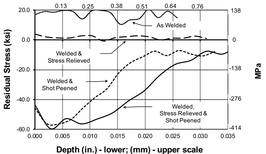
Fig. 3-1 Residual Stresses from Welding
