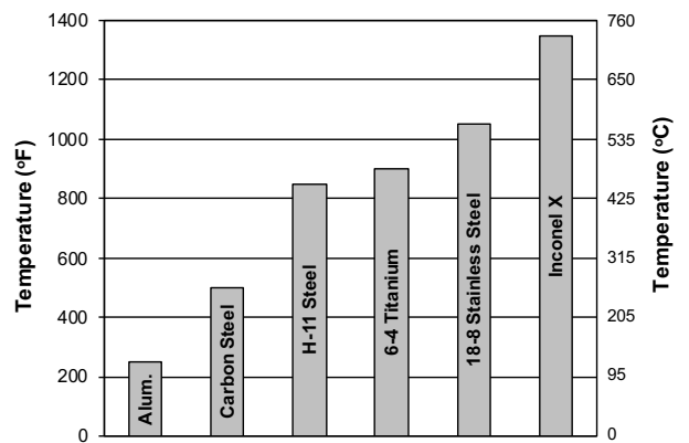
Fig. 9-2 Approximate Temperature at Which Compressive Stresses Begin to Dissipate
