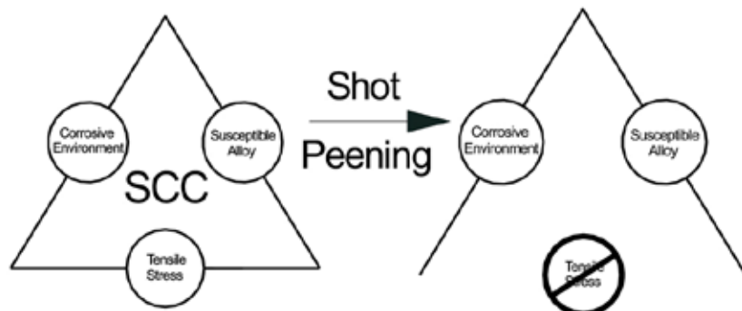
Fig. 8-1 Stress Corrosion Cracking Triangle
