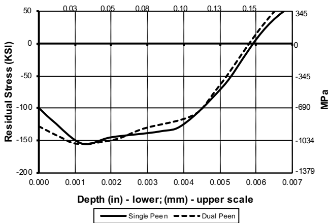
Fig. 10-11 Single Peen vs Dual Peen
