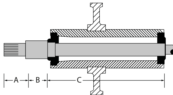
Fig. 11-11 Assembly Drawing of Splined Shaft Requiring Shot Peening
