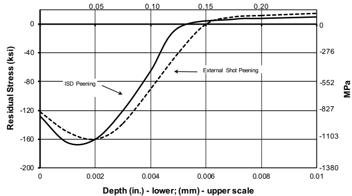
Fig. 10-10 Internal Surface Deflector vs External Shot Peening
