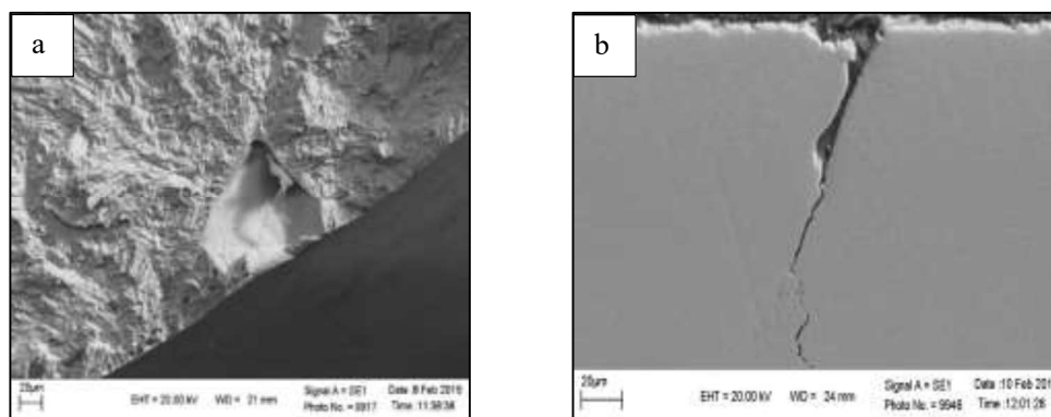
Plate 3 - Surface Failure from a) Cold Shut/Oxide Film and b) Micro-section showing a Fatigue Crack Initiating from a Cold Shut
