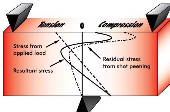
Shot peening influence on applied stress
