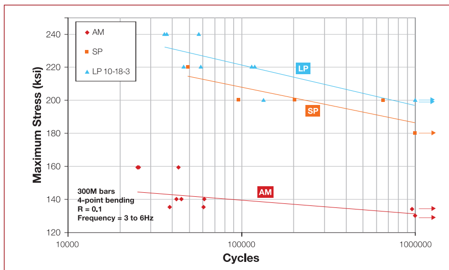
Figure 3. Effect of laser and shot peening on the fatigue lifetime of 4-pt bend bars with Kt=1. Both treatments are highly effective in increasing the fatigue strength for this smooth surface case where surface stress is critical to prevent initiation.
