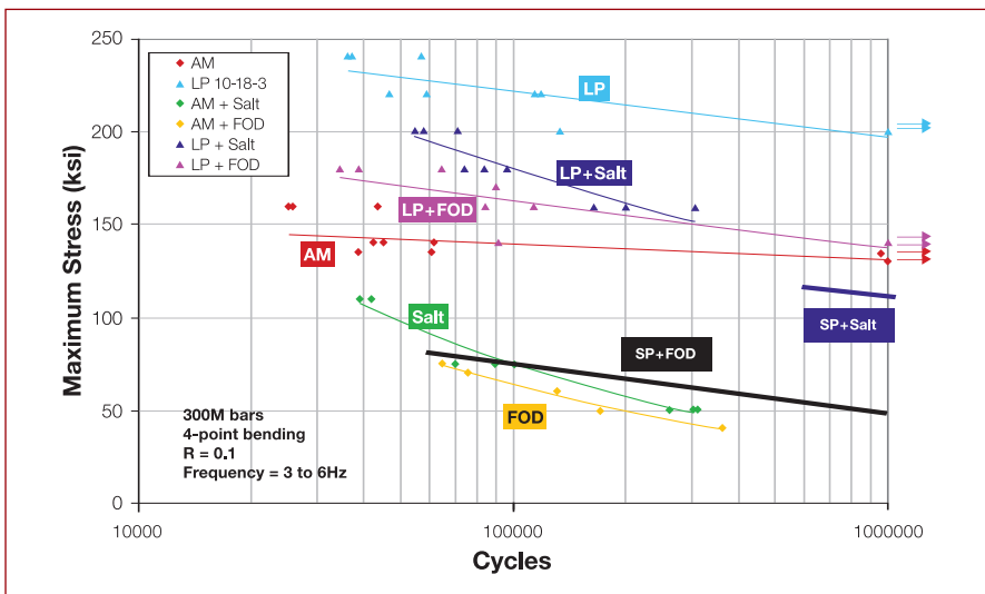
Figure 5. Deep level of residual stress generated by laser peening dramatically distinguishes it from shot peening in the presence of damage such as FOD or salt corrosion.
