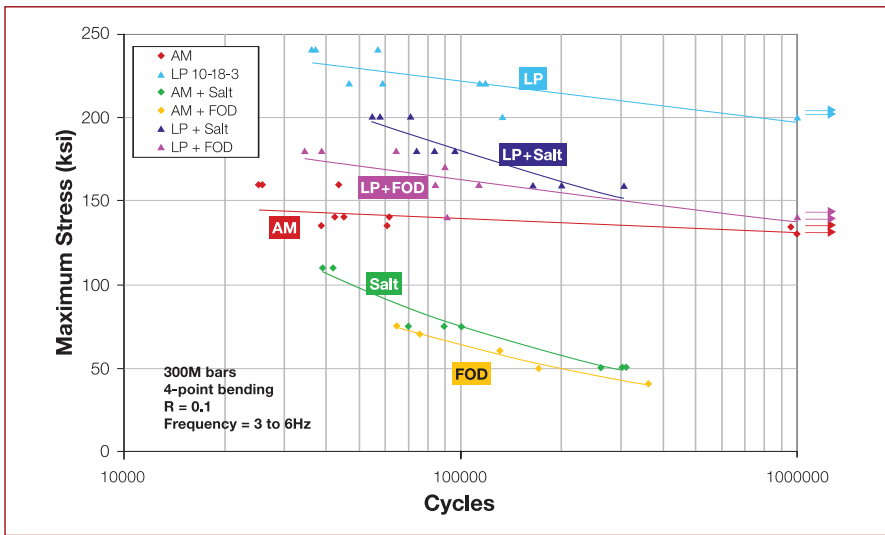
Figure 4. Stress-lifetime curve for laser peened and as machined samples damaged by a 0.020-inch notch cut into the high stress region of the sample using an EDM wire or corrosion simulated by alternate exposure to a 3.5% salt bath. The lack of surface compressive stresses results in rapid deterioration of the AM samples whereas the laser peened samples show more than 250% advantage in fatigue strength.
