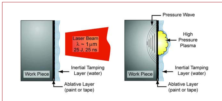
Figure 1. In the laser peening process, ablation of a sacrificial layer at the surface of the part creates a high-pressure plasma and consequent shock wave that results in a deep compressive stress in the workpiece.
