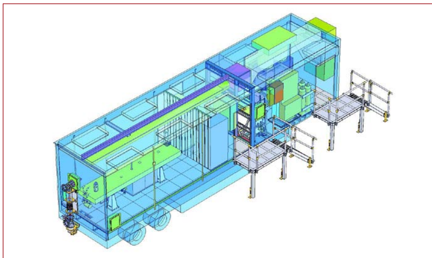
Figure 7. The laser peening system has been packaged into a transportable system for remote processing applications. Requiring only electrical power, a fully equipped peening system can be rapidly set up at field sites for overhaul and repair work.
