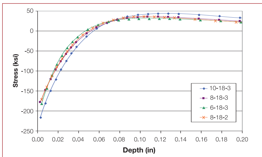
Figure 2. Compressive stress developed by laser peening in 300M in a 0.5-inch-thick sample not corrected for sample bending.
