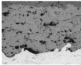
Typical Microstructure of Porous Thermal Barrier Coating (TBC)
